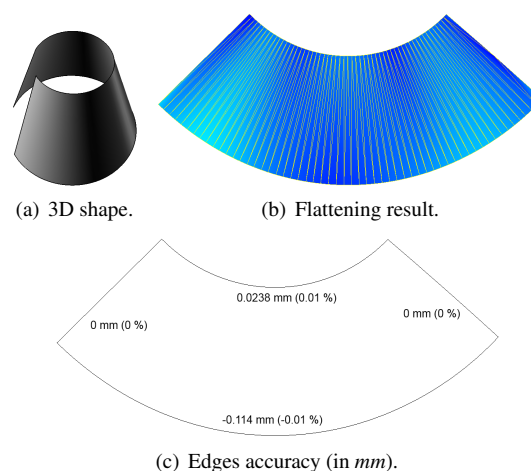
Figure 1: Developable surface - a cone.
