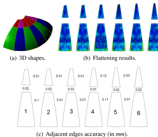
Figure 2: Examples of well developable surfaces.
