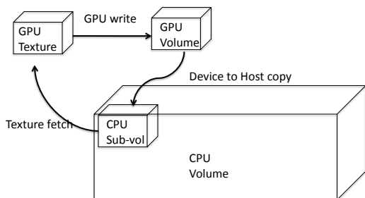
Figure 2: Streaming computation.
