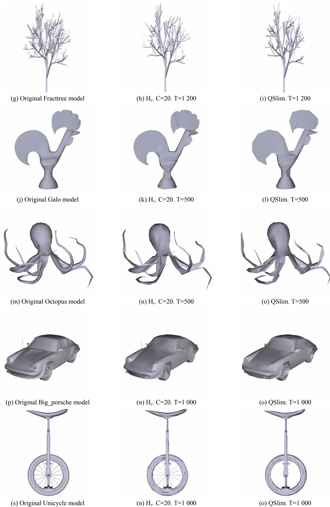
Figure 5. Results for all models. C indicates the number of viewpoints and T the number of triangles
