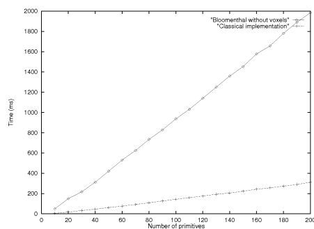
Figure 7: Tessellation times
