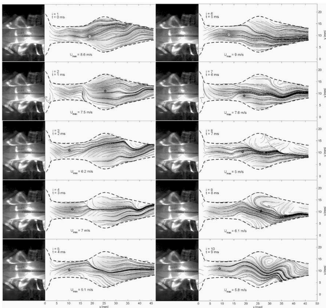
Fig. 5. Airflow streamlines measured in the model of the glottal region for vowel /a:/ and the snapshots of the self-oscillating vocal folds (left part of the panels) registered at the time instants corresponding to the time steps i = 1 - 10 in Fig. 3. The air flows from left to right. ( Q_{\text{mean}} = 0.21 l/s, P_{\text{sub}} = 940 Pa, F_0 = 180 Hz)
