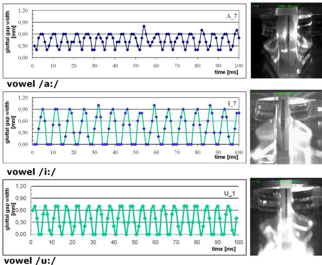
Fig. 3. Measured glottal gap in time domain (left) evaluated for all vowels at each time instant from the images of the self-oscillating vocal folds (right)
