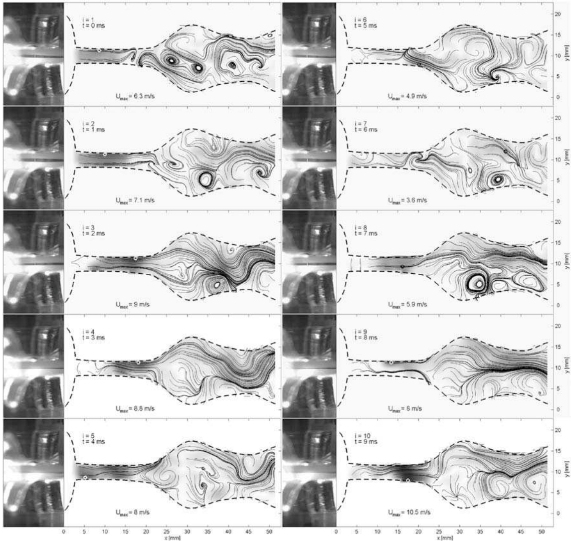
Fig. 7. Airflow streamlines measured in the model of the glottal region for vowel /u:/ and the snapshots of the self-oscillating vocal folds (left part of the panels) registered at the time instants corresponding to the time steps i = 1 - 10 in Fig. 3. The air flows from left to right. ( Q_{\text{mean}} = 0.21 l/s, P_{\text{sub}} = 930 Pa and F_0 = 192 Hz)
