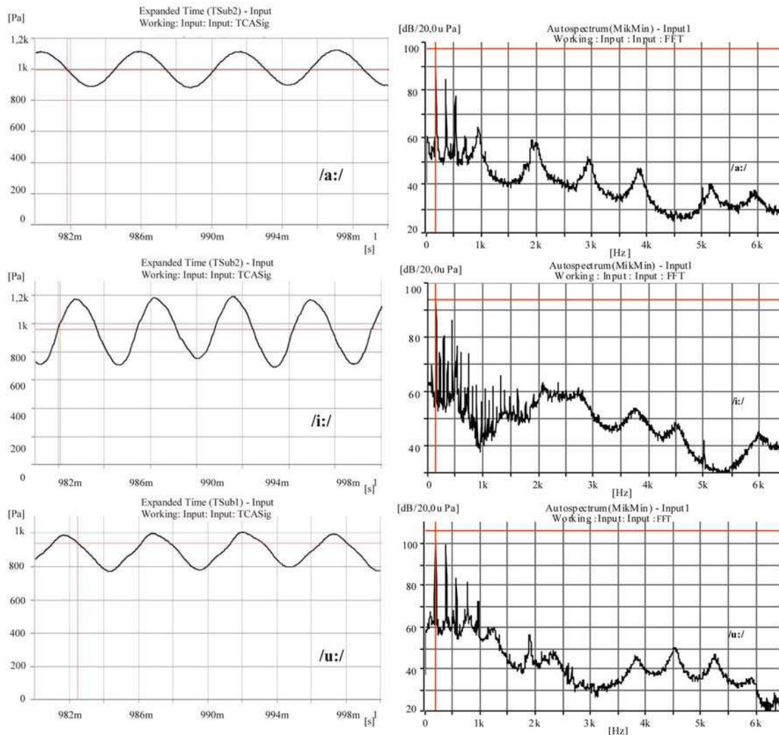
Fig. 4. Measured subglottal pressure for vowels /a:/, /i:/ and /u:/ (left) and spectra of the microphone signal at the mouth models (right)
