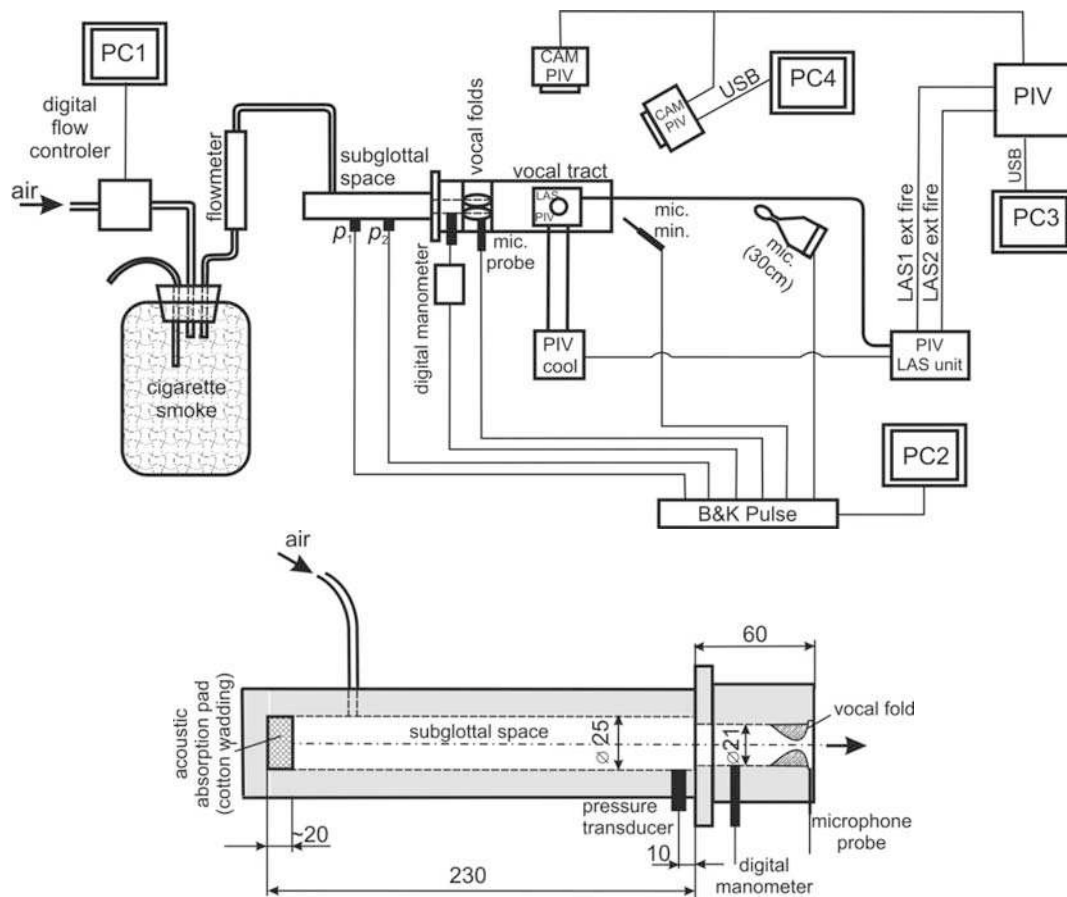
Fig. 1. Schematic simplified measurement set-up and a detail of the subglottal and glottal part
