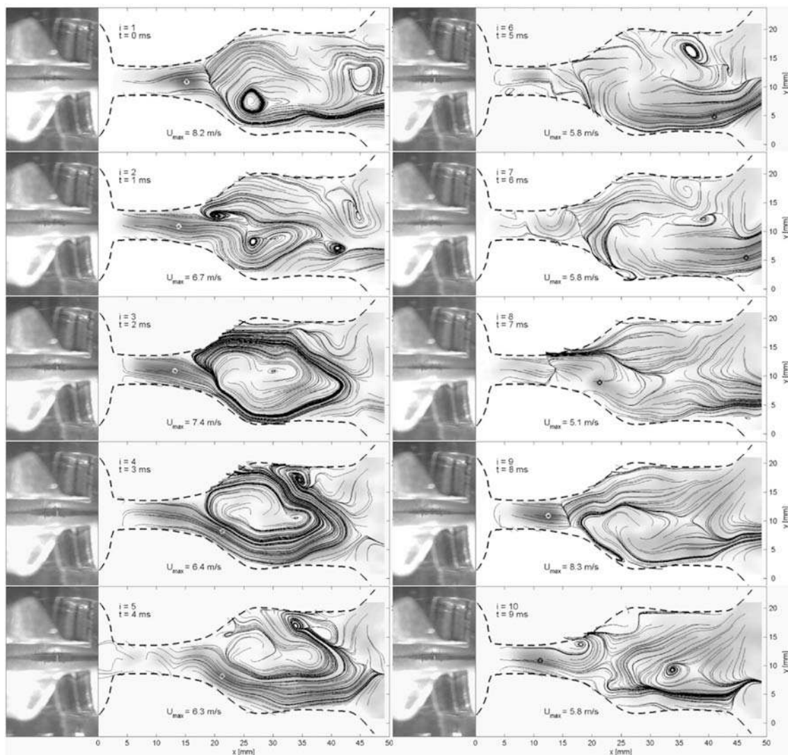
Fig. 6. Airflow streamlines measured in the model of the glottal region for vowel /i:/ and the snapshots of the self-oscillating vocal folds (left part of the panels) registered at the time instants corresponding to the time steps i = 1 - 10 in Fig. 3. The air flows from left to right. ( Q_{\text{mean}} = 0.24 l/s, P_{\text{sub}} = 910 Pa, F_0 = 148 Hz)
