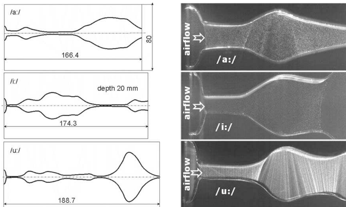
Fig. 2. Models of the human vocal tract for vowels /a:/, /i:/ and /u:/ (left) and field of view of the glottal region with flowing particles in the PIV laser light (right)
