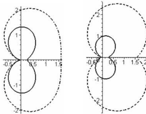
Fig. 1. Plastic zone estimation for the plane stress (dashed line) and plane strain (solid line) states for Mises (left) and Tresca (right) yield criteria (courtesy of S. Seitzl [20])
