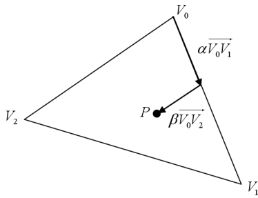
Figure 3: Parametric representation of the ray-triangle intersection point P .
