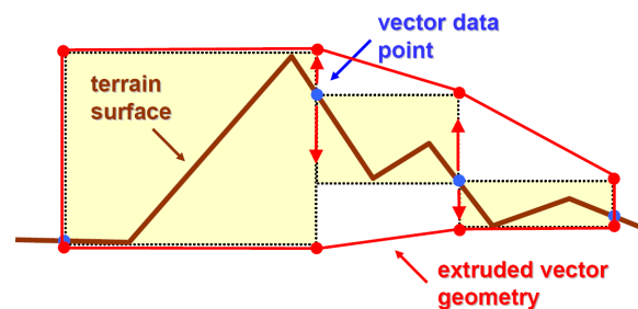
Figure 3: A 2d diagram of the extrusion of a linestrip. The original vector data points (blue) are duplicated and moved to the upper and lower bounds of the line segments bounding box constituting the top and bottom caps (red).
