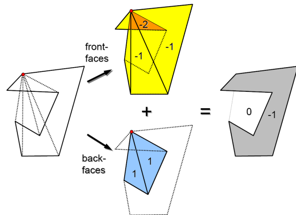
Figure 5: Tessellation of a concave polygon into a convex fan creating a concave mask in the stencil buffer.
