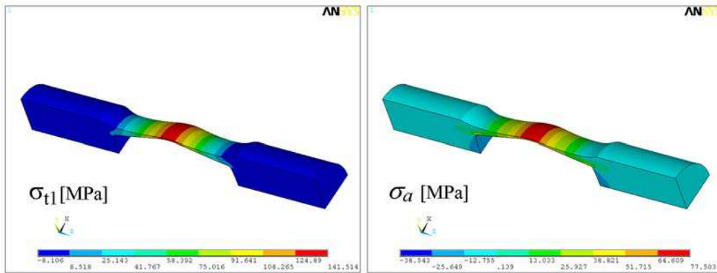
Fig. 4. Circumferential and axial stresses for inner overpressure 15 MPa
