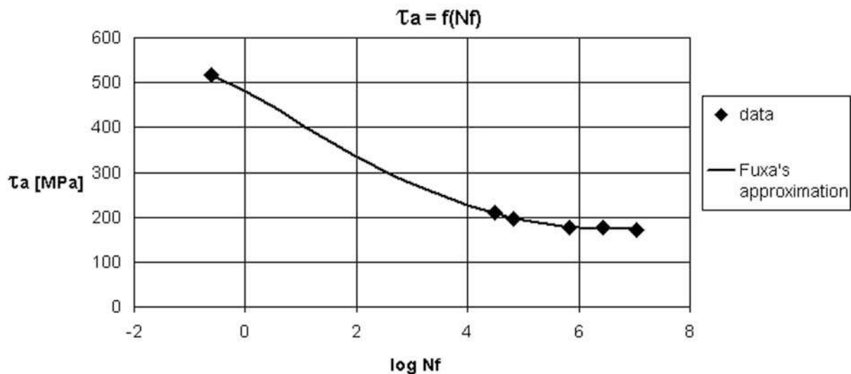
Fig. 2. S-N – curve for alternating torsion
