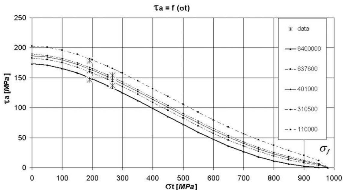
Fig. 3. Fuxa’s approximation for combined torsion – tension loading
