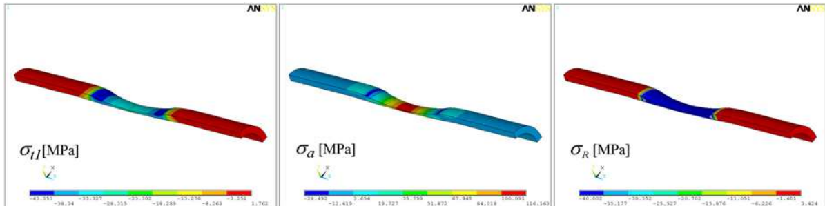
Fig. 6. Circumferential, axial and radial stresses for inner and external overpressure 40 MPa in specimen – Nr. 2. in tab. 4
