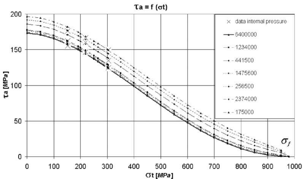
Fig. 5. Fuxa's approximation for combined torsion – inner overpressure loading
