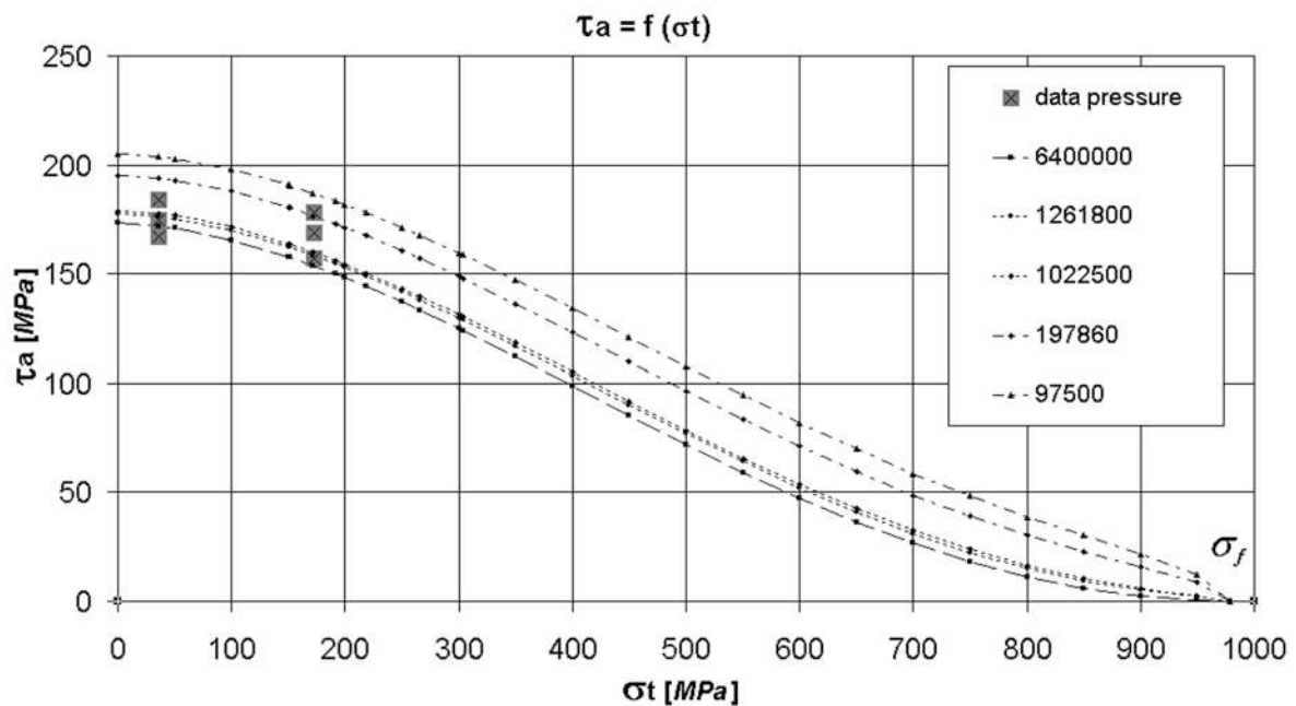
Fig. 7. The Fuxa’s approximation for combined loading by torsion – inner, external overpressure and axial force
