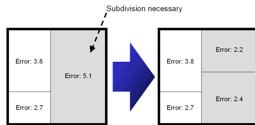
Figure 9: Subdivision: A cell will be partitioned if the error is worse compared to the error of the other cells.
