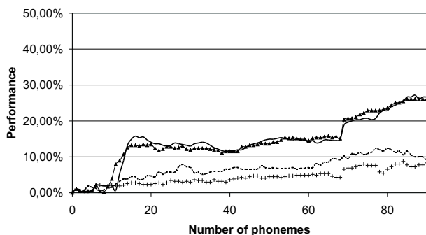
Figure 7: Speaker identification performance when the training data came from the desk microphone and the test data from the close-talking microphone. Dashed line = identification based on the likelihood of the whole utterance; line of crosses = identification based on the majority voting rule for single phonemes; solid line = identification based on the majority voting rule for sequences of 10 phonemes; line of triangles = identification based on the majority voting rule for sequences of 7 phonemes.
