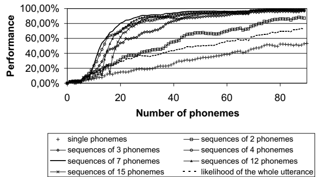
Figure 4: Determination of the optimal number of phonemes for the procedure based on the majority voting rule for sequences of phonemes.
