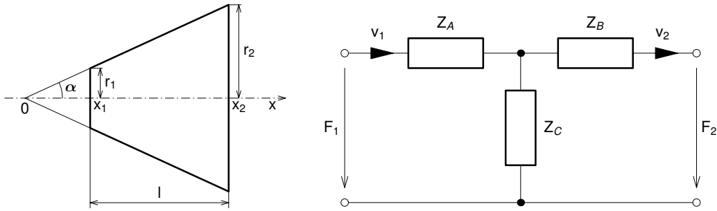
Fig. 3. A conical divergent waveguide (left), an equivalent circuit (right)
