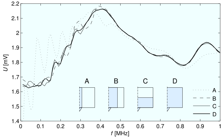
Fig. 9. Influence of backing geometry on the frequency response
