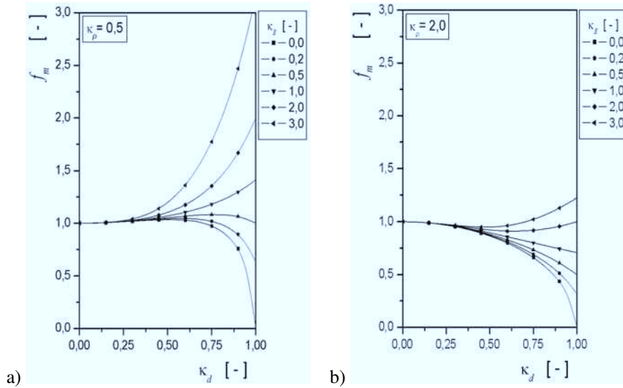
Fig. 2. The dependency of modification function f_m of beam type I on \kappa_d parameter for different parameters \kappa_E and fixed parameter, a) \kappa_\rho = 0,5 ; b) \kappa_\rho = 2,0
