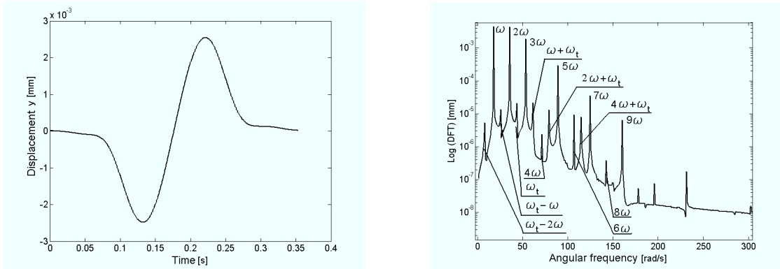
Fig. 12. Time domain response in horizontal direction of a cracked rotor system with torsional excitation (left) and corresponding frequency domain response (right).
