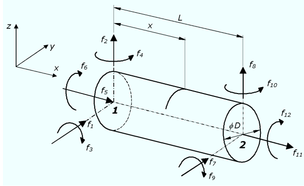
Fig. 1. A shaft element with the transverse crack.
