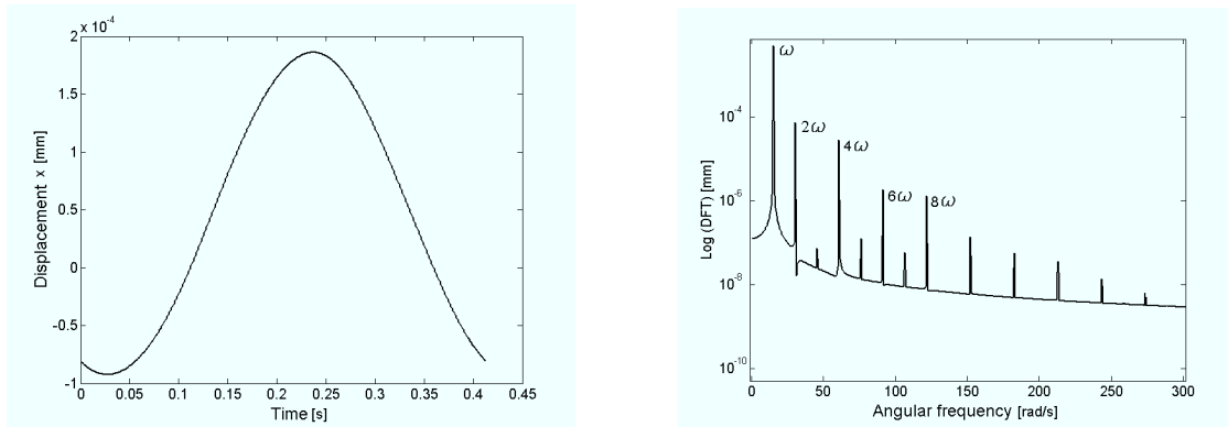
Fig. 9. Time domain response in axial direction of a cracked rotor system (left) and corresponding frequency domain response (right).
