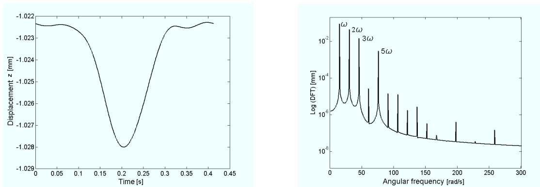
Fig. 8. Time domain response in vertical direction of a cracked rotor system (left) and corresponding frequency domain response (right).
