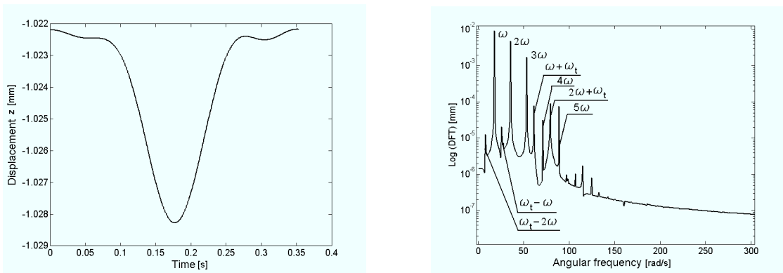
Fig. 13. Time domain response in vertical direction of a cracked rotor system with torsional excitation (left) and corresponding frequency domain response (right).
