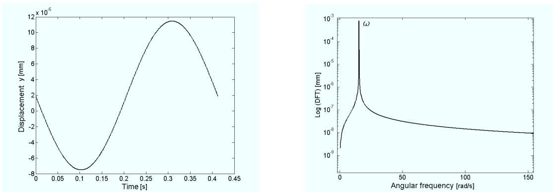
Fig. 4. Time domain response in horizontal direction of an uncracked rotor system with torsional excitation (left) and corresponding frequency domain response (right).
