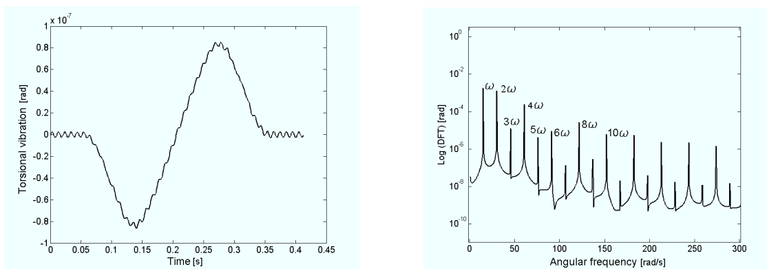
Fig. 10. Time domain torsional response of a cracked rotor system (left) and corresponding frequency domain response (right).
