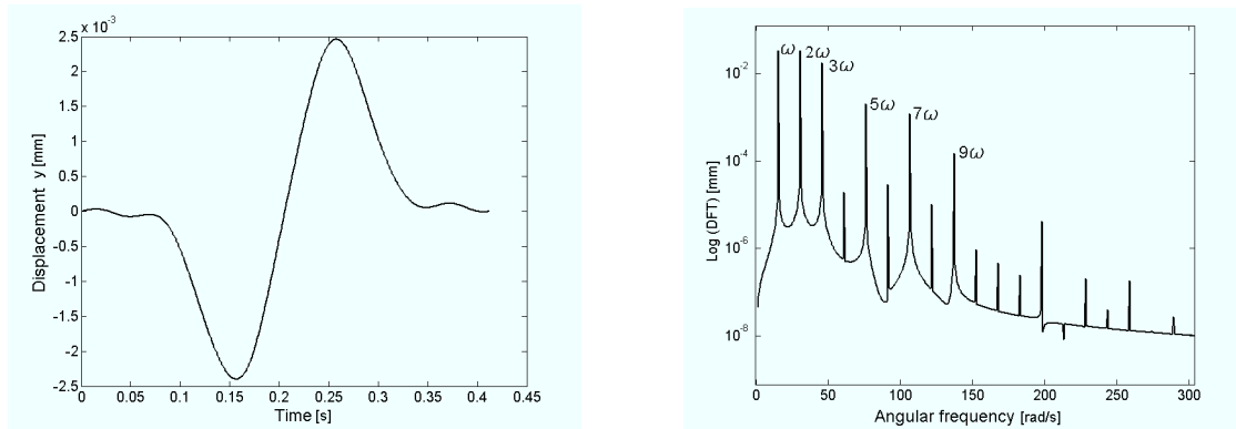
Fig. 7. Time domain response in horizontal direction of a cracked rotor system (left) and corresponding frequency domain response (right).
