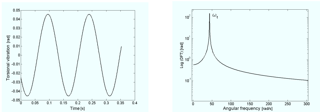
Fig. 15. Time domain torsional response of a cracked rotor system with torsional excitation (left) and corresponding frequency domain response (right).
