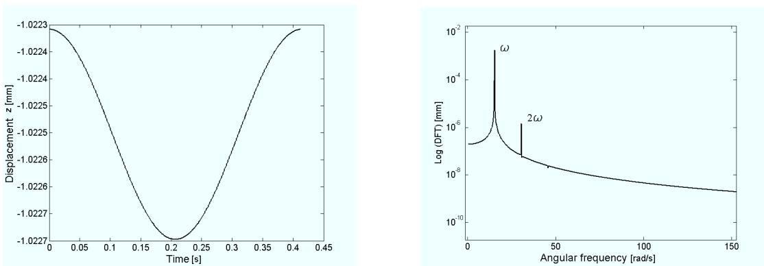
Fig. 5. Time domain response in vertical direction of an uncracked rotor system with torsional excitation (left) and corresponding frequency domain response (right).
