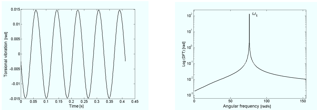
Fig. 6. Torsional response in time domain of an uncracked rotor system with torsional excitation (left) and corresponding frequency domain response (right).
