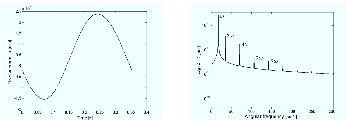
Fig. 14. Time domain response in axial direction of a cracked rotor system with torsional excitation (left) and corresponding frequency domain response (right).
