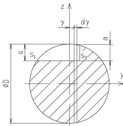
Fig. 2. The cross-section of shaft with the crack.
