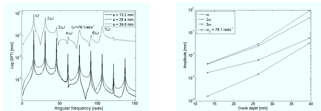
Fig. 11. Frequency domain response in horizontal direction of a cracked rotor system (left) and variation of amplitudes of rotational frequency and its higher harmonics (right).
