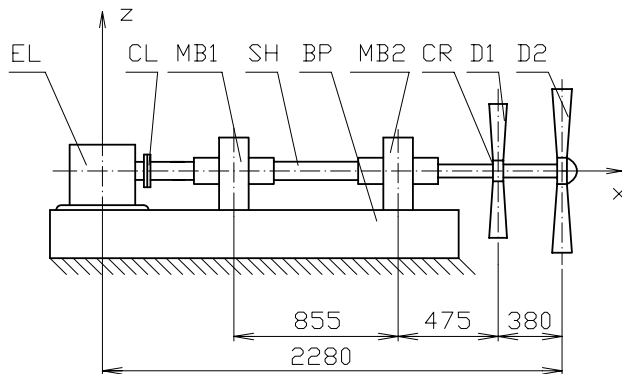
Fig. 3. A sketch of the test rotor system.
