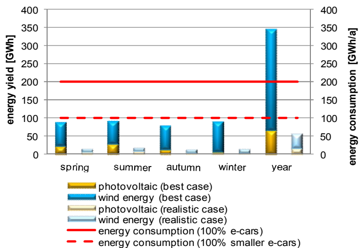
Figure 5 – Comparison of the required energy with the total yield of renewable energy systems
