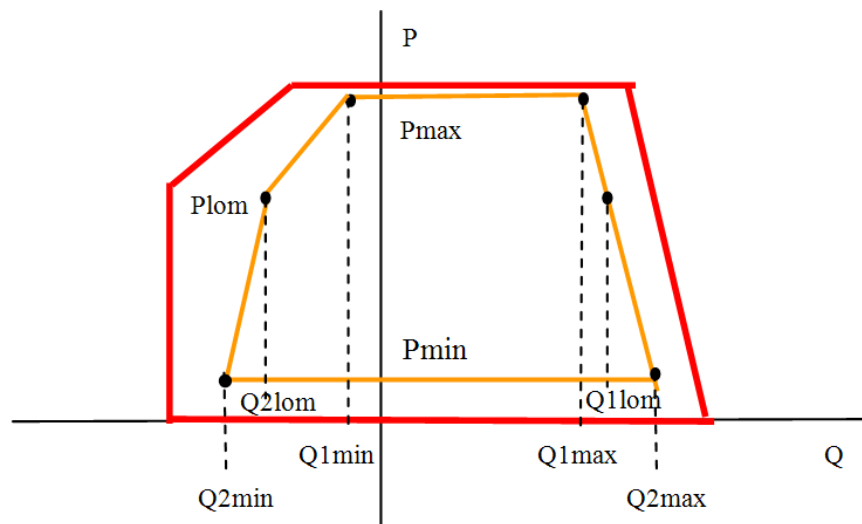
Fig. 1 Operational chart of the generator
