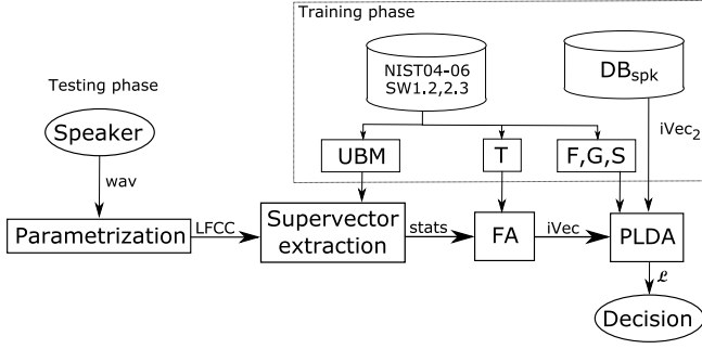
Fig. 1. Diagram of the verification process with four steps: parametrization, supervector extraction, dimensionality reduction by FA and finally verification with another speaker (represented as iVector) using PLDA model. The output from the PLDA system is likelihood ( \mathcal{L} ) that two iVectors (new constructed iVec and iVec 2 from databases DB spk ) representing the same speaker.
