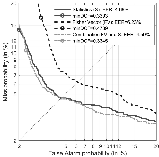
Fig. 2. DET curves of comparison systems: the system using Suprvector of Statistics (S) or FV and a combination of these two systems. Circles denote points where minDCF occurred. Dotted line indicates EER.
