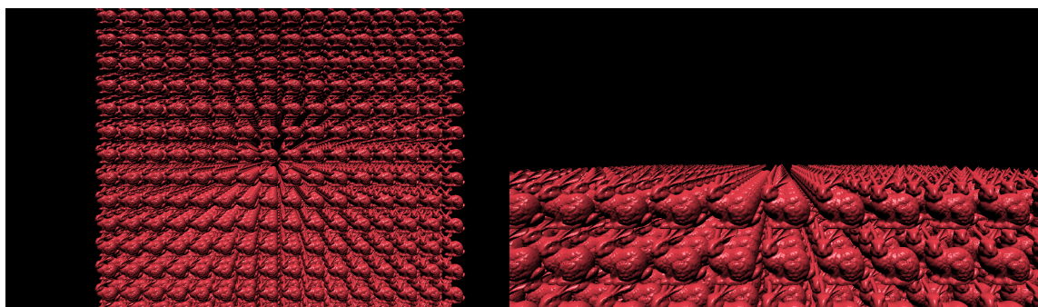
Figure 9: Rendering results using Screen Space Billboard Voxel Buffer in 720p with Nvidia Geforce GTX 980. Test scene contains 4096 Stanford Bunny which are represented by about 10 billion voxels (20 billion triangle in base algorithm). We achieved about 70 FPS for the left image and about 160 FPS for the right image.
