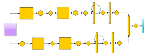
Figure 5: 2-column C3D joined at input and output.
