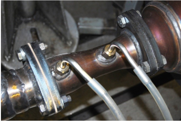
Figure 3. Narrowed exhaust pipeline for velocity measuring
