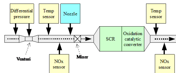
Figure 1. Block diagram of exhaust system
