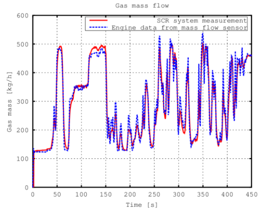
Figure 5. The comparison of mass flow measurement methods
