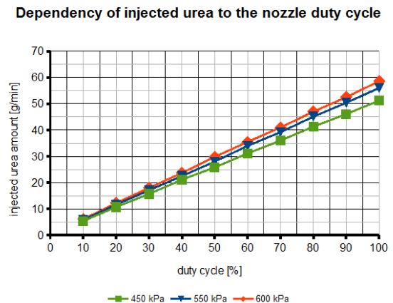
Figure 6. The urea amount dependency on the duty cycle
