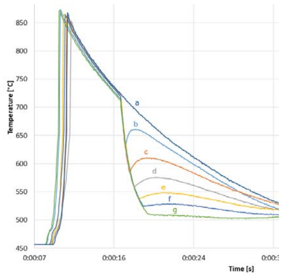
Figure 6. Cooling by air with different process time
