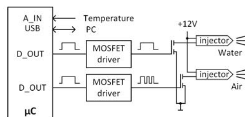
Figure 1. Block diagram of the driving circuit
