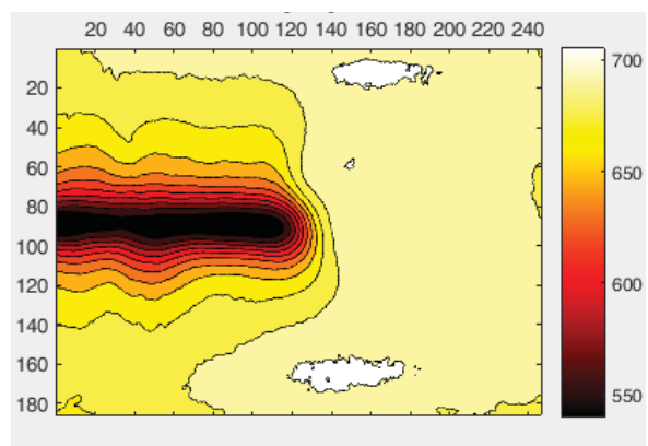
Figure 8. Temperature distribution –developed linear nozzle
