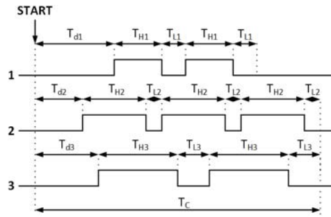
Figure 3. Waveform of driving signals
