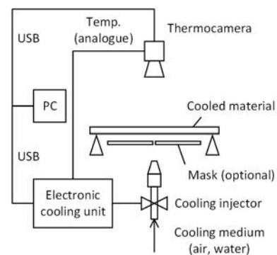
Figure 4. Measuring stand
