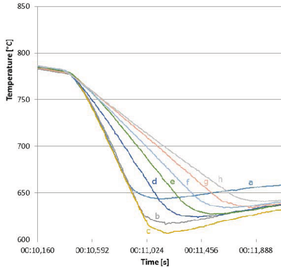
Figure 5. Cooling by water with different duty cycle
