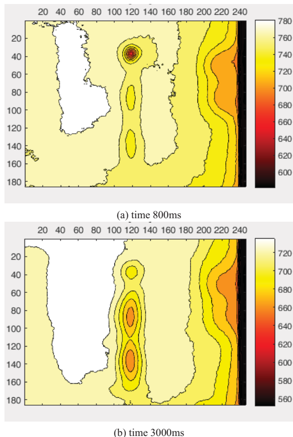
Figure 7. Temperature distribution – 3 injectors with a mask
