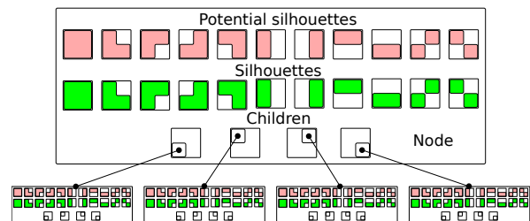
Figure 6: Node data in 2D space for the 8-bit compression. One node contains sets of silhouette and potentially silhouette edges, each addressed by its bitmask value. If a set shape does not intersect the triangle planes of an edge, the edge is stored into the set. The largest set shape is chosen if multiple set shapes do not intersect the triangle planes. A node also contains pointers to child nodes.
