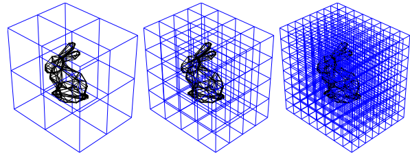
Figure 4: The algorithm supports a custom level of voxelization. The image shows three levels (1,2,3) of depth of the octree for the same scale of the scene bounding box.
