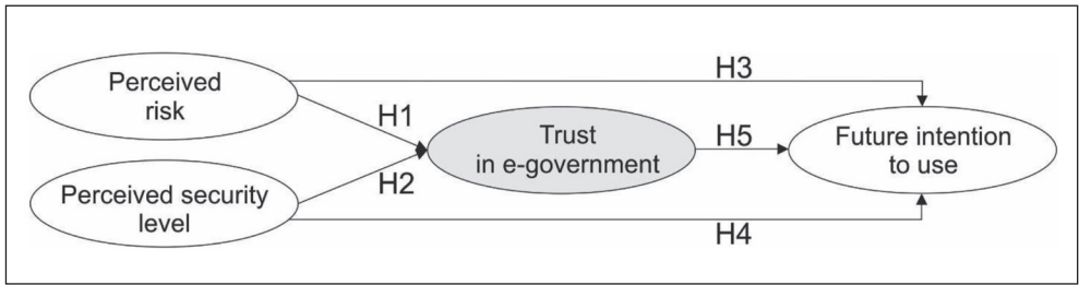
Fig. 1: Conceptual model
