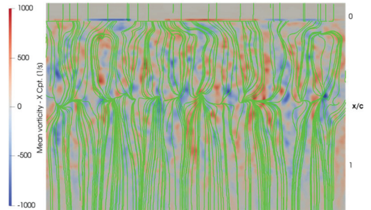
Fig. 7. Plane y_w/c = 0.01 m . Mean spanwise vorticity contours and surface vector lines of mean velocity.
