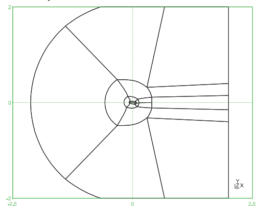
Fig. 1. The blocking structure of the mesh axes ticks in metres while the plate has chord of 0.1 m.
