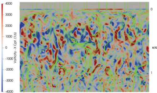
Fig. 5. Plane y_w/c = 0.01 m . Instantaneous spanwise vorticity contours and surface vector lines of instantaneous velocity.
