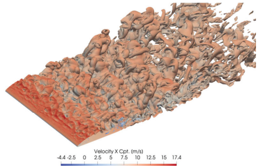
Fig. 15. Iso-surface of instantaneous vorticity 500 1/s. Coloured by streamwise velocity.
