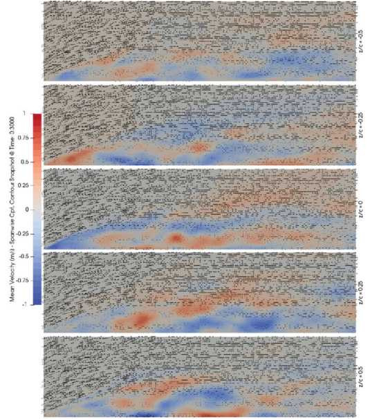
Fig. 6. Spanwise normal planes above plate suction surface. Mean spanwise velocity contours and vectors of mean in-plane velocity.
