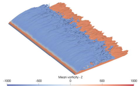
Fig. 16. Iso-surface of mean vorticity 500 1/s. Coloured by its spanwise oriented component.
