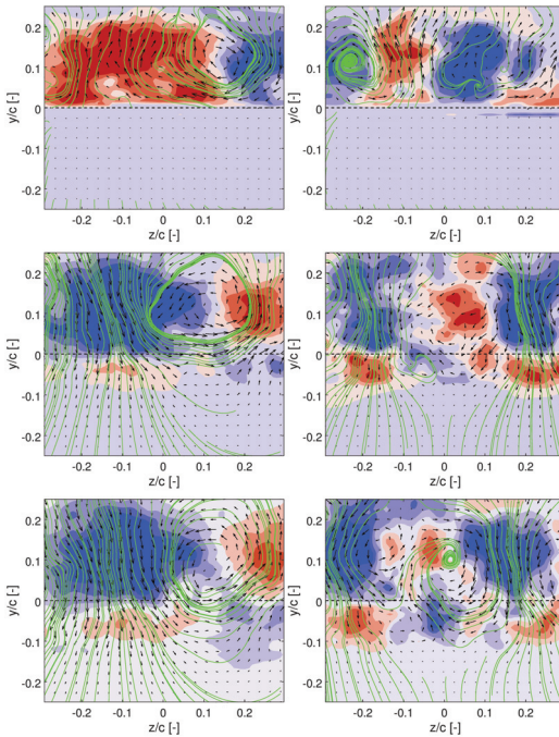
Fig. 12. Parts of streamwise normal planes x/c = 1, 1.3, 1.5 (top to bottom). POD modes of velocity no. 1 (left) & 4 (right). Content \sim 4.6\% & \sim 3.2\% of TKE.
