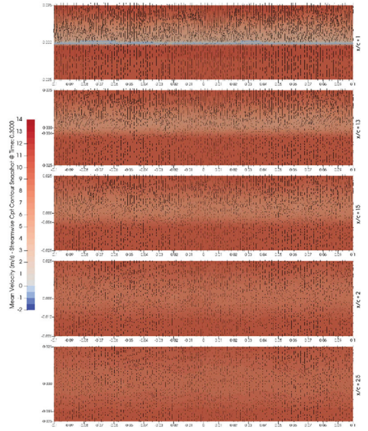
Fig. 13. Streamwise normal planes above plate suction surface. Mean spanwise velocity contours and vectors of mean in-plane velocity.
