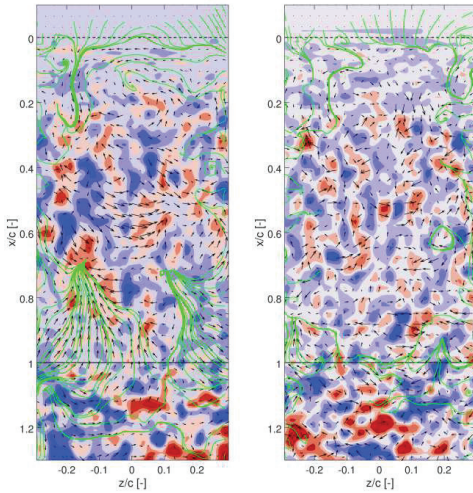
Fig. 9. Spanwise slices of plane y_w/c = 0.01 m . Velocity POD modes no. 6 (left) & 46 (right). Content 2.3% & 1.2% of TKE.
