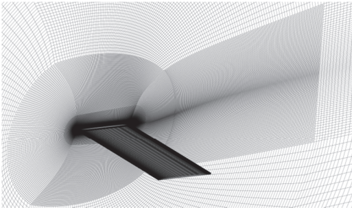
Fig. 2. Detail of the cut-cell refined mesh in the vicinity of the flat plate.
