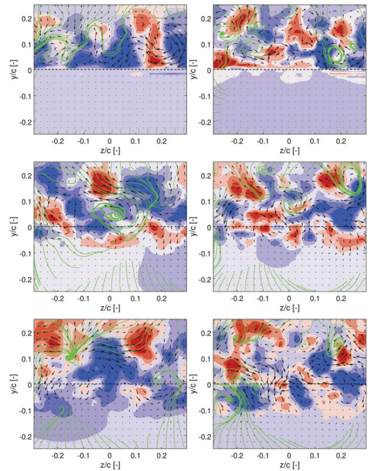
Fig. 14. Parts of streamwise normal planes x/c = 1, 1.3, 1.5 (top to bottom). POD modes of velocity no. 7 (left) & 17 (right). Content \sim 2.5\% & \sim 1.8\% of TKE.
