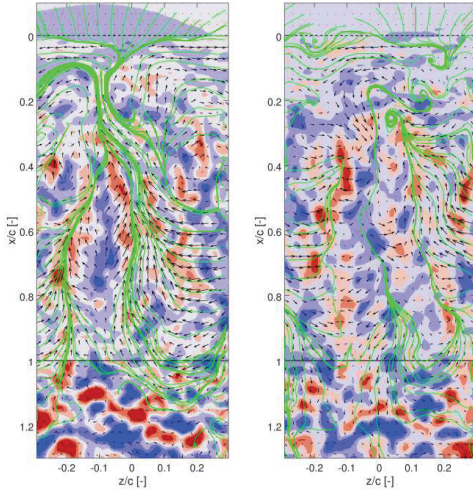
Fig. 8. Spanwise slices of plane y_w/c = 0.01 m . Velocity POD modes no. 1 (left) & 2 (right). Content 3.1% & 2.8% of TKE.
