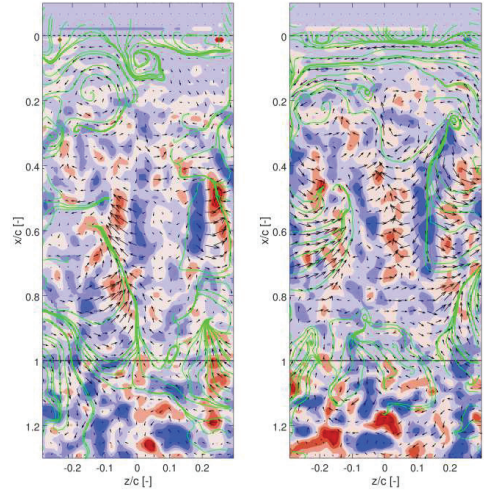
Fig. 10. Spanwise slices of plane y_w/c = 0.01 m . Velocity POD modes no. 3 (left) & 5 (right). Content 2.5% & 2.3% of TKE.
