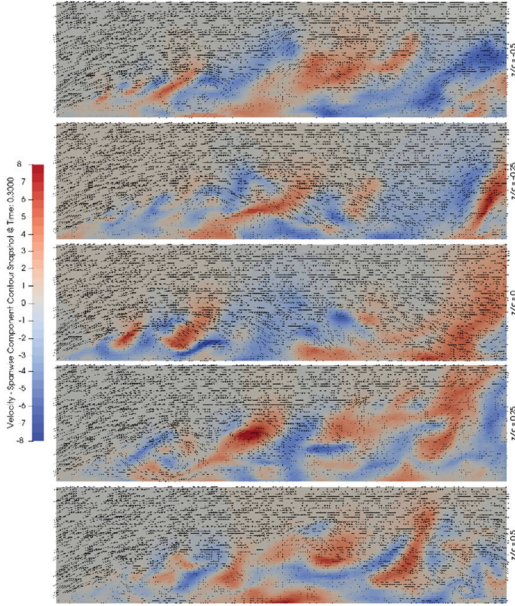
Fig. 4. Spanwise normal planes above plate suction surface. Instantaneous spanwise velocity contours and vectors of instantaneous in-plane velocity.
