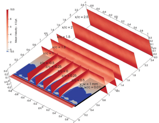
Fig. 3. Sampling planes annotated, mean velocity streamwise component plotted. Plate surface rendered black.
