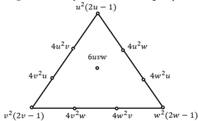
Figure 2. Cubic Timmer basis functions.
