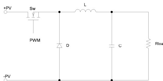
Figure 4. Schematic diagram of the ideal buck converter
