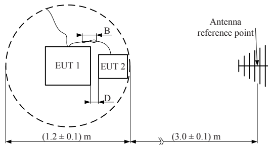
Figure 3. Test area of small device for radiated emission measurement – top view
