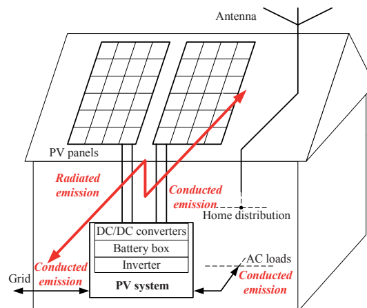
Figure 1. Block diagram of the PV system across the house
