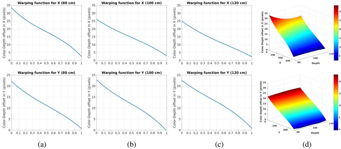
Figure 8: Warping functions W^x and W^y for different distances for the Orbbec Astra Pro sensor. (a): 80cm calibration distance. (b): 100cm calibration distance. (c): 120cm calibration distance. (d): Interpolated warping functions S^x (top) and S^y (bottom).
