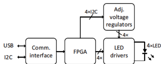
Figure 1. PDD block diagram
