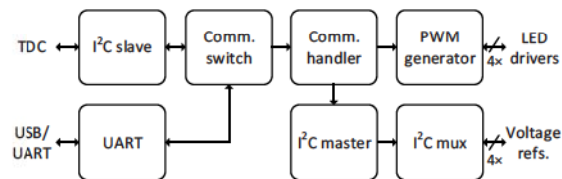
Figure 4 Block diagram of firmware
