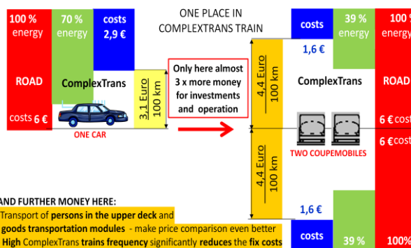
FIG.11 – the energy and price comparison of rail transport of a conventional car and a coupemobile shows why coupemobiles for transport in the train are much more economical. It is possible to get much more money from one place when transporting coupemobiles instead of common cars.
