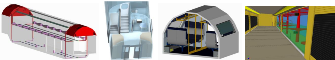
FIG.3 – double-deck railway coach of the ComplexTrans system - the upper floor serves for passengers and the lower floor is used for freight transport modules and passenger cars (coupemobiles). There are boarding areas, staircases and sanitary facilities at the ends of the coach.
