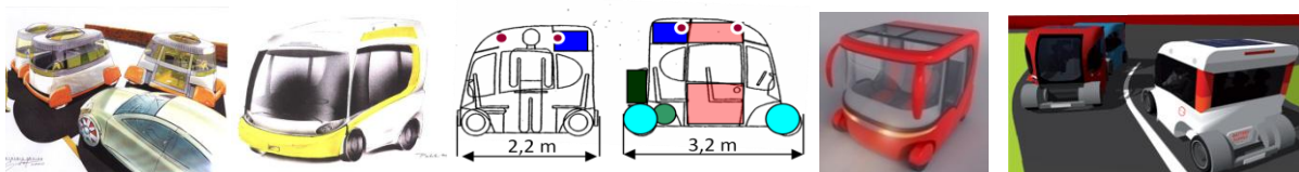
FIG. 5 - Several design pictures of a coupemobile. With the axles retracted, the length of the vehicle is only 2.2 m, while the wheelbase is increased by 1 m while driving. It is possible to enter the trains laterally and to park perpendicular to the pavement.
