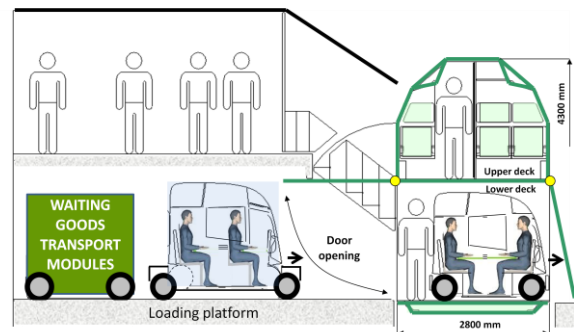
FIG.7 – cross-section through the two-story platform of the ComplexTrans system. The lower deck serves for loading and disloading of passenger cars and waiting freight transport modules. The car crew remains in their coupemobiles during the rail transport as in a rail coupé. The other passengers are transported on the upper deck, where they come from the second floor of the platform by folding doors with stairs located at the ends of the coaches.
