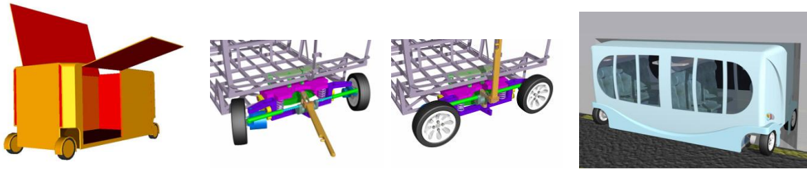
FIG.4 - The freight and passenger transport modules are equipped with its own low power electric drive for independent local manipulation. The wheels can be swiveled 90 ° for lateral loading into the railcoach.
