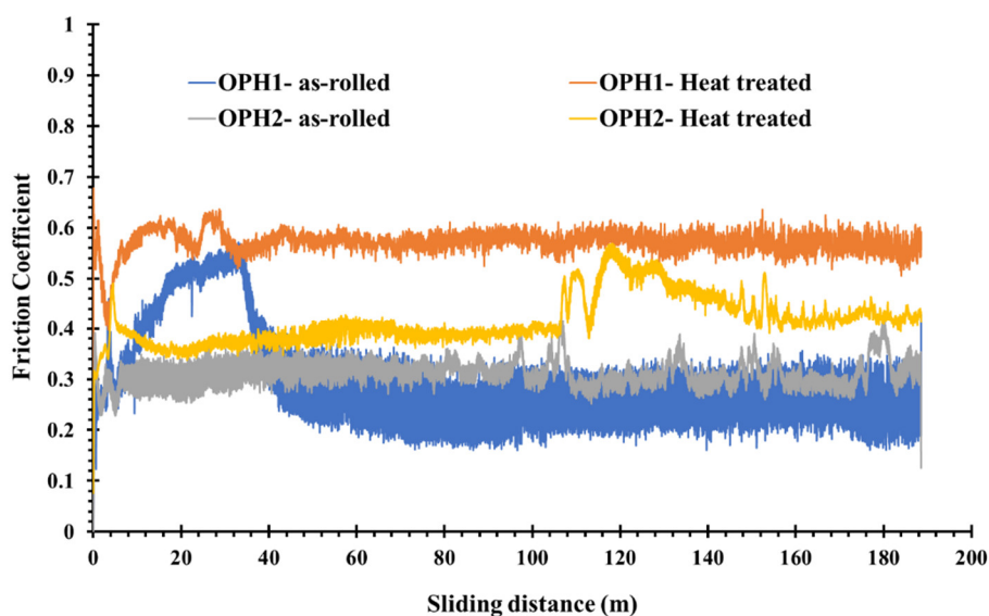
Figure 10. Friction coefficient vs. sliding distance during the pin-on-disk test.
