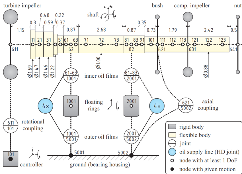
Figure 1. Schematic representation of the analyzed turbocharger. Depicted lengths and diameters are dimensionless; dimensionless length 1 corresponds to ca. 8.5 mm
