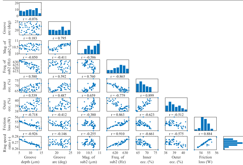
Figure 5. Correlation matrix for the turbine bearing at rotor speed 60 krpm
