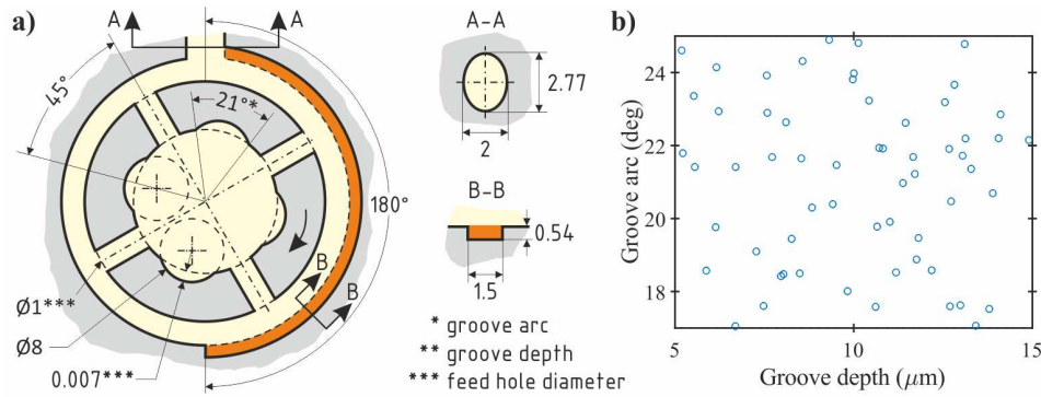
Figure 2. (a) Dimensioned drawing of the floating ring bearing, dimensions are in mm; (b) distribution of random variables
