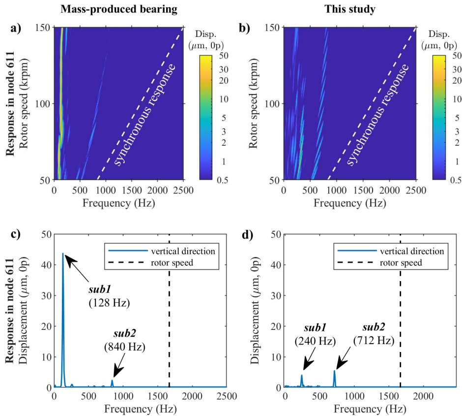
Figure 3. (a, b) FFT of the steady-state response at speeds {50; 60; ... 150} krpm and (c, d) FFT of the steady-state response at 100 krpm
