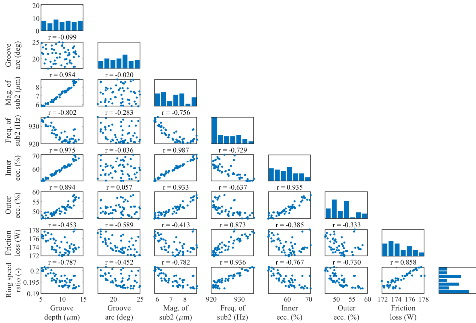
Figure 7. Correlation matrix for the turbine bearing at rotor speed 130 krpm
