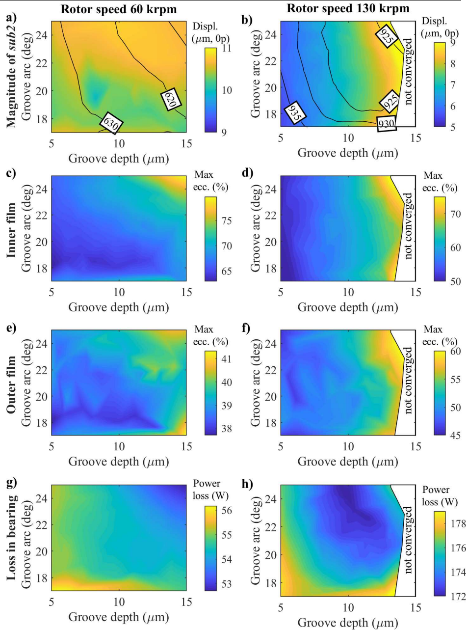
Figure 4. Relationships of various output parameters in the turbine bearing on the groove depth and arc; labels shown in Figures 4a and 4b represents the frequency of sub2 component
