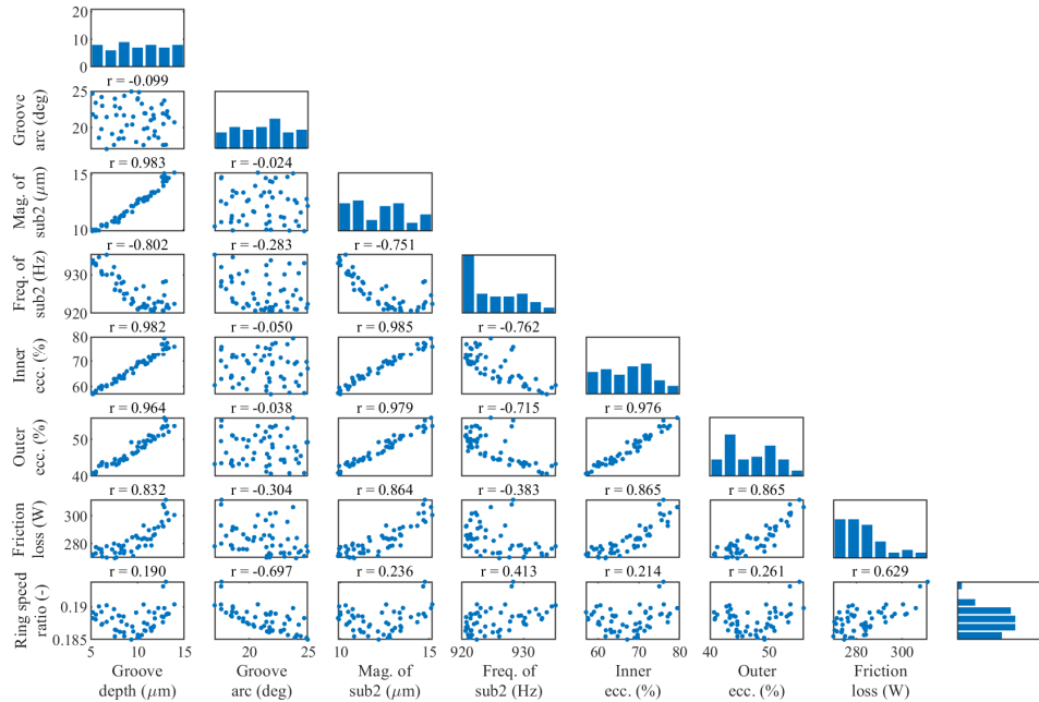
Figure 8. Correlation matrix for the compressor bearing at rotor speed 130 krpm
