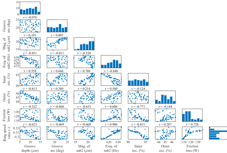
Figure 6. Correlation matrix for the compressor bearing at rotor speed 60 krpm
