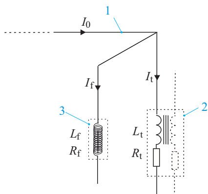
Fig. 6. Distribution of the quasi-direct current I_0 into the current I_f passing through the frequency filter 3 and into the current I_t in the high-voltage winding of the transformer 2
