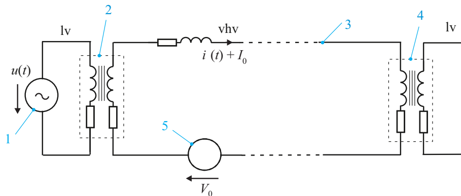
Fig. 2. Simple model of single-phase electrical supply system: 1 – generator, 2 – step-up power transformer, 3 – very high voltage transmission line, 4 – step-down power transformer, 5 – source of quasi-variable voltage induced by magnetic storm
