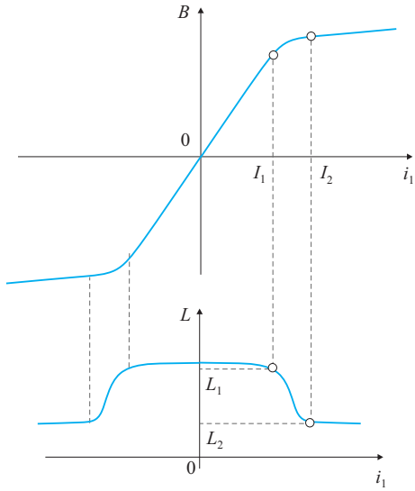
Fig. 4. The course of inductance of the power transformer winding during supersaturation of its magnetic circuit
