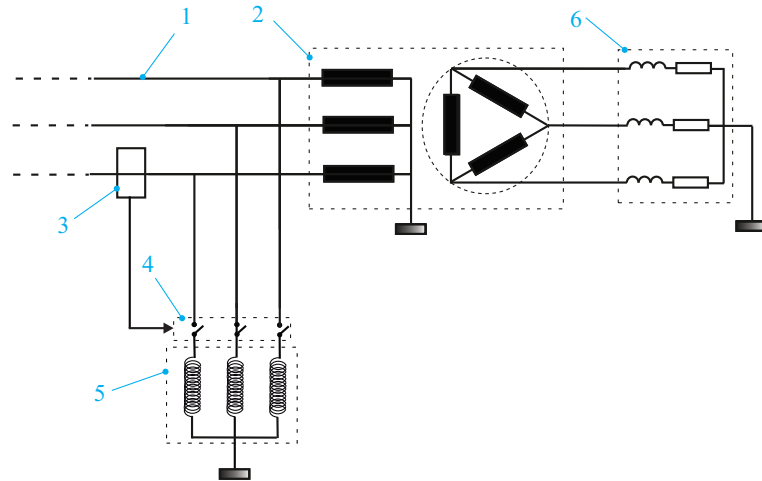
Fig. 7. Connection of a three-phase superconducting reactor to the high-voltage side of a step-down power transformer in a YD connection, converting electrical power into the distribution network: 1 – high voltage transmission line, 2 – three-phase step-down power transformer in YD connection with zero output, 3 – indicator of quasi-stationary current I_0 in high voltage transmission line, 4 – switch to connect/disconnect superconducting reactor in the transmission system, 5 – three-phase superconducting reactor in connection Y with output zero, 6 – three-phase distribution network simulated by three-phase impedance in connection Y with ground
