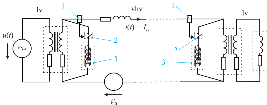
Fig. 5. A simple model of a single-phase electrical supply system, whose power transformers are protected by superconducting reactors: 1 – sensor-indicator of the quasi-stationar current I_0 in the high voltage transmission line, 2 – a switch that connects/disconnects the superconducting reactor to the high voltage winding of the power transformer, 3 – single-phase superconducting reactor
