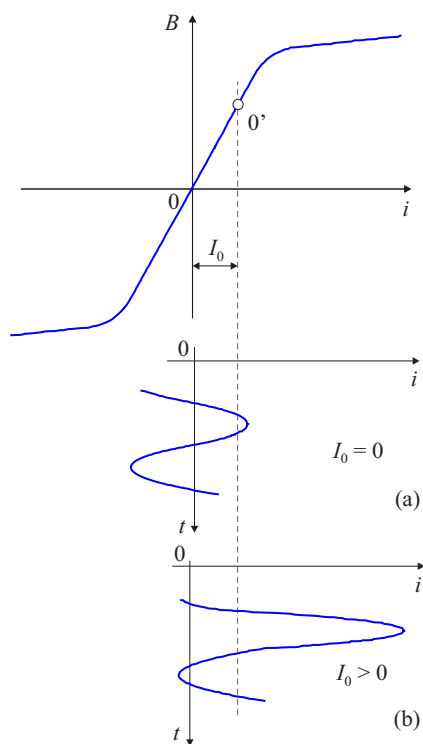
Fig. 3. Influence of supersaturation of the magnetic circuit of the power transformer on the occurrence of current overload the phenomenon of semisaturation of the magnetic circuit of the power transformer: (a) – without supersaturation, (b) – with supersaturation
