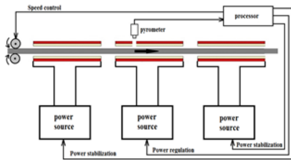
Fig.1. Diagram of the control system of a modular induction heater of the second type with a single control point
