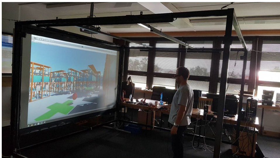
Fig. 3 Setup of CAVE with participant performing the experiment (Color figure online)
