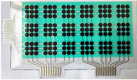
Figure 1. Sample with circular electrodes
