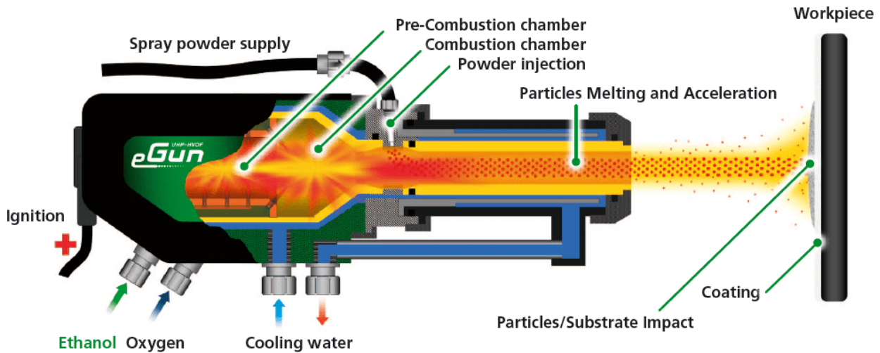
Fig. 2. Scheme of equipment for creating a coating by HVOF technology [4]
