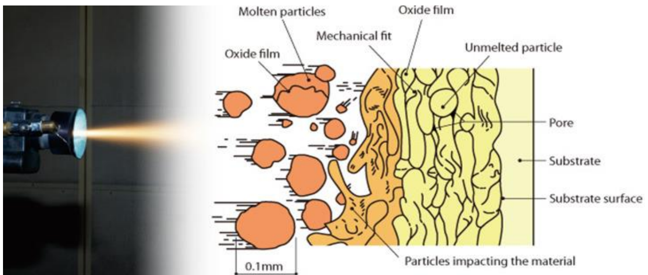
Fig. 1. Description of the HVOF spray application principle [9]
