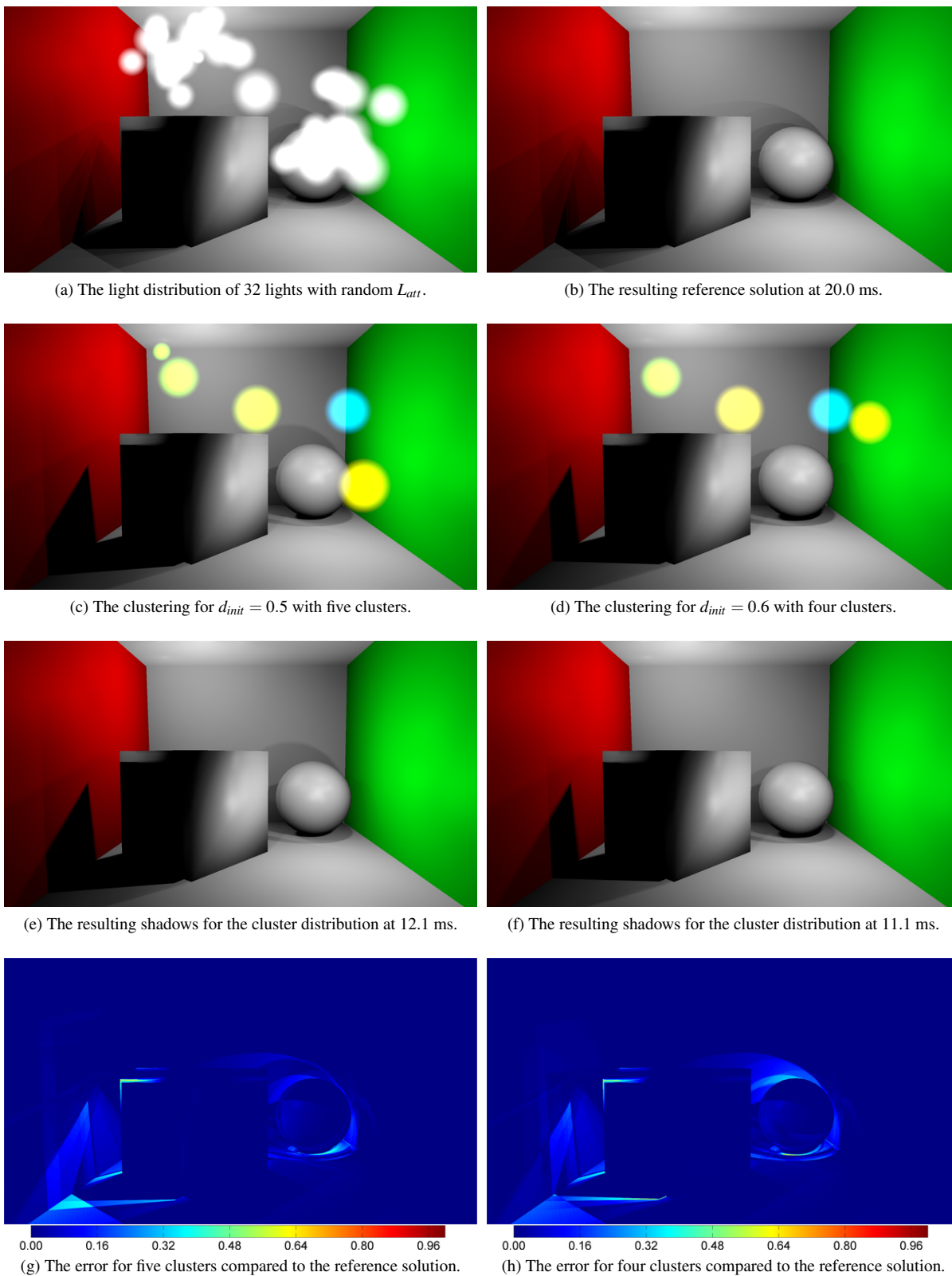
Figure 8: Comparison for the Cornell Box scene.
