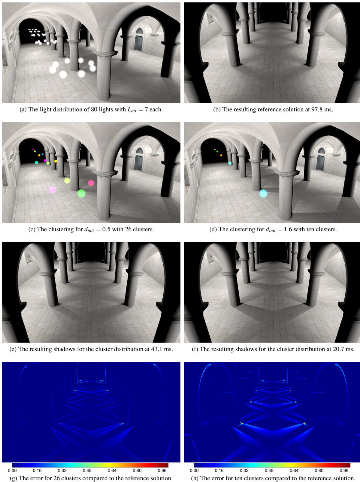
Figure 7: Comparison for the Dabrovic Sponza scene.
